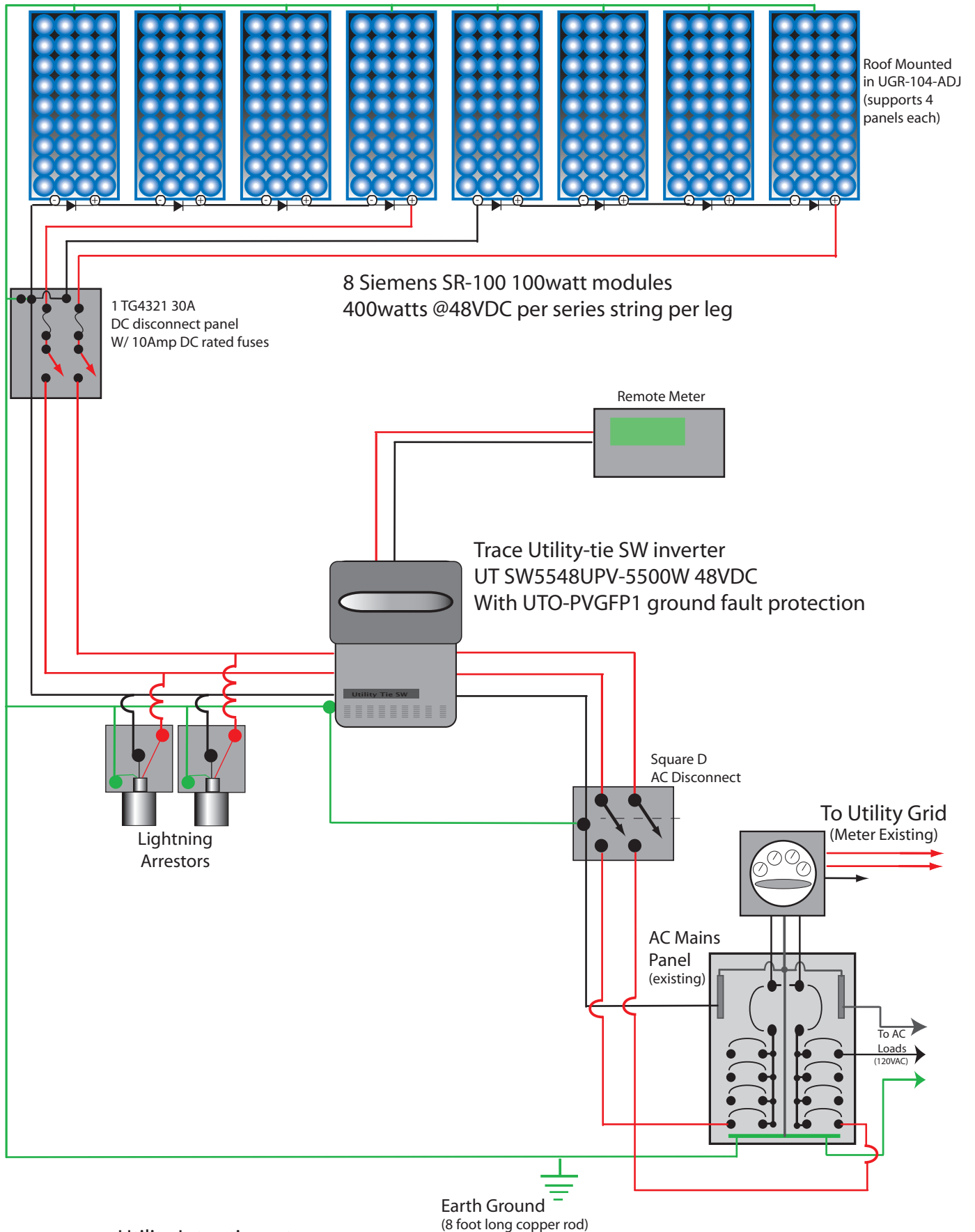
Utility Inter-tie system By Gerald Zack
